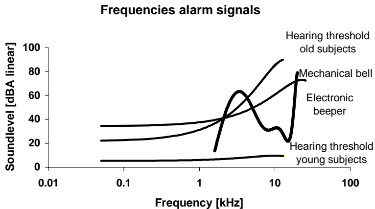
Figure 1 Schematic sound spectra of beeper and mechanical bell as compared to average hearing thresholds of young and old subjects.
